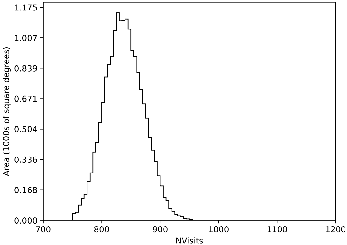
ddf_loaded_half_fl8_v3.4_10yrs WFD all bands: NVisits
