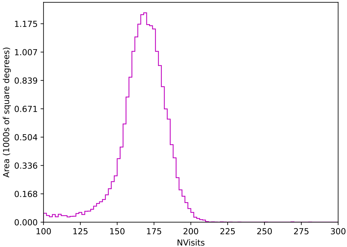
ddf_loaded_half_fl8_v3.4_10yrs All sky z band: NVisits
