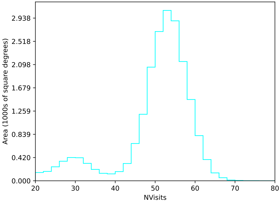
ddf_loaded_half_fl8_v3.4_10yrs All sky u band: NVisits
