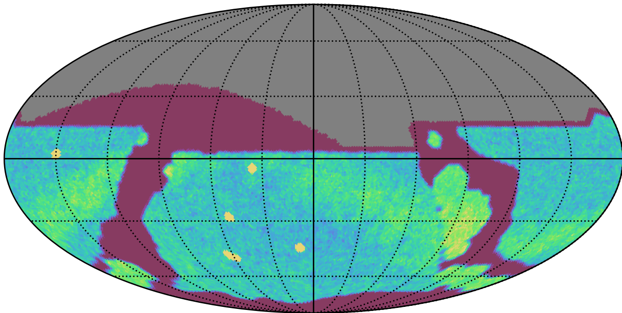
ddf_loaded_half_fl8_v3.4_10yrs All sky r band: NVisits
