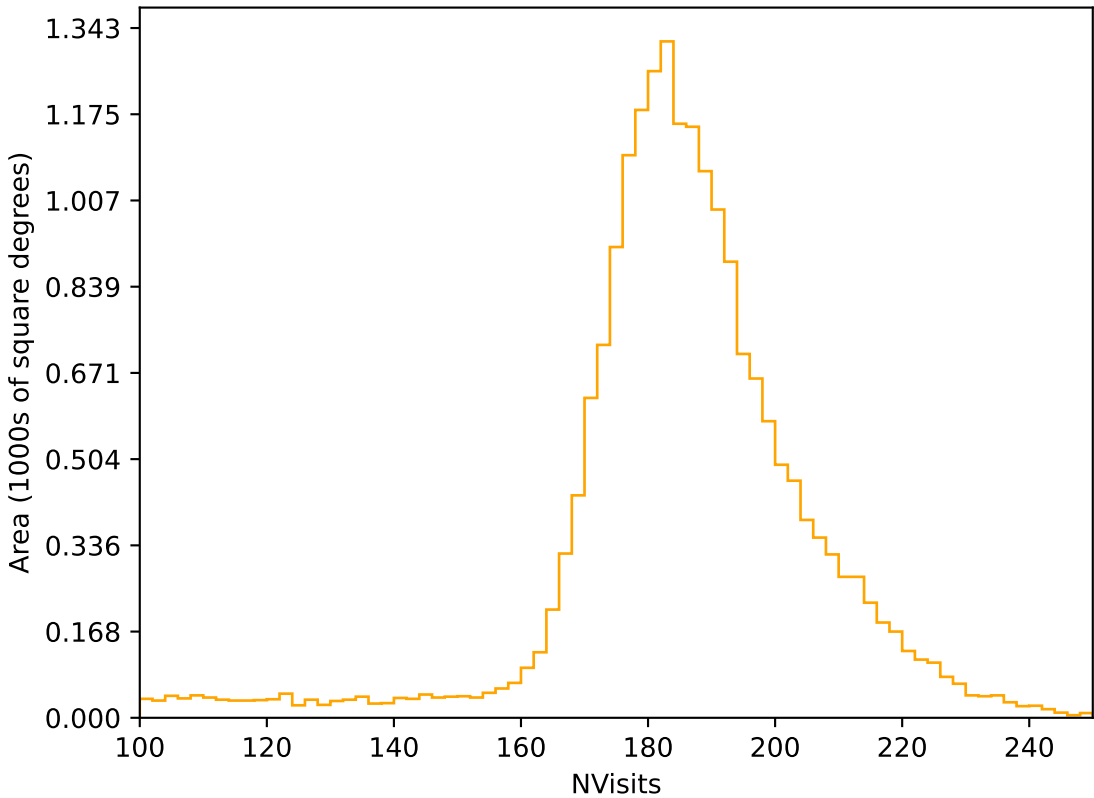
ddf_loaded_half_fl8_v3.4_10yrs All sky r band: NVisits
