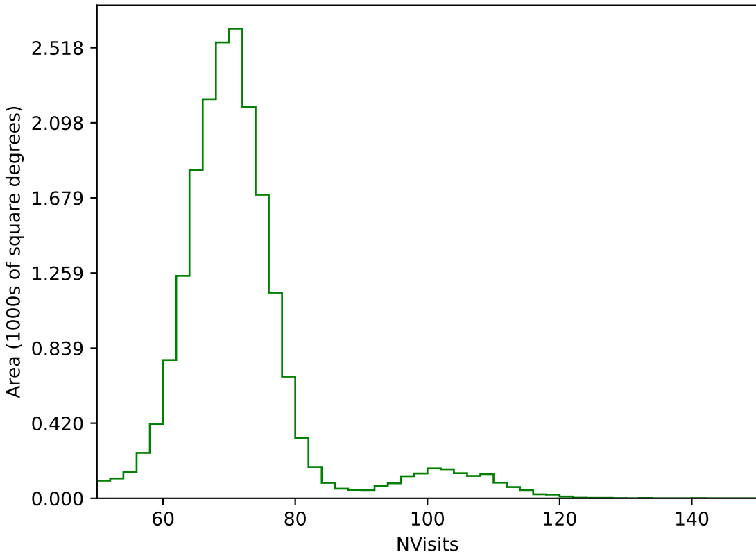
ddf_loaded_half_fl8_v3.4_10yrs All sky g band: NVisits
