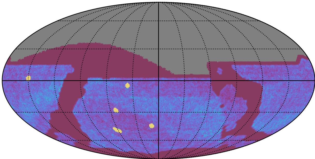
ddf_loaded_half_f18_v3.4_10yrs All sky all bands: NVisits
