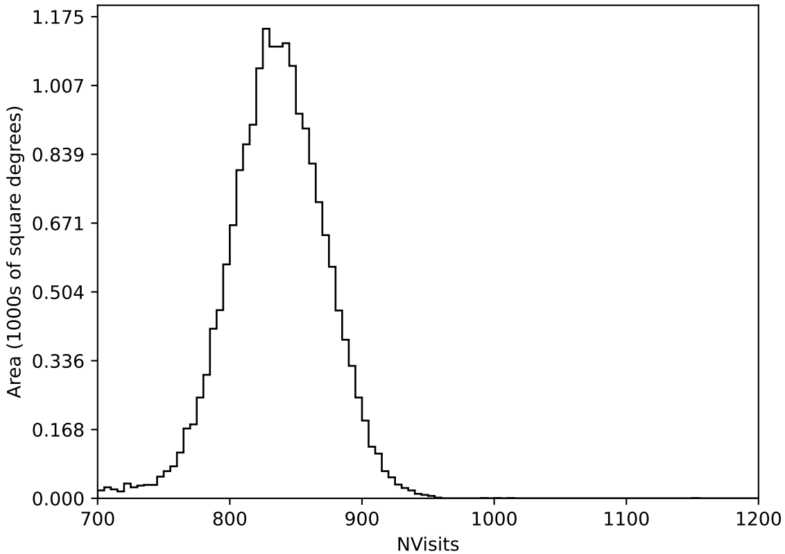
ddf_loaded_half_fl8_v3.4_10yrs All sky all bands: NVisits
