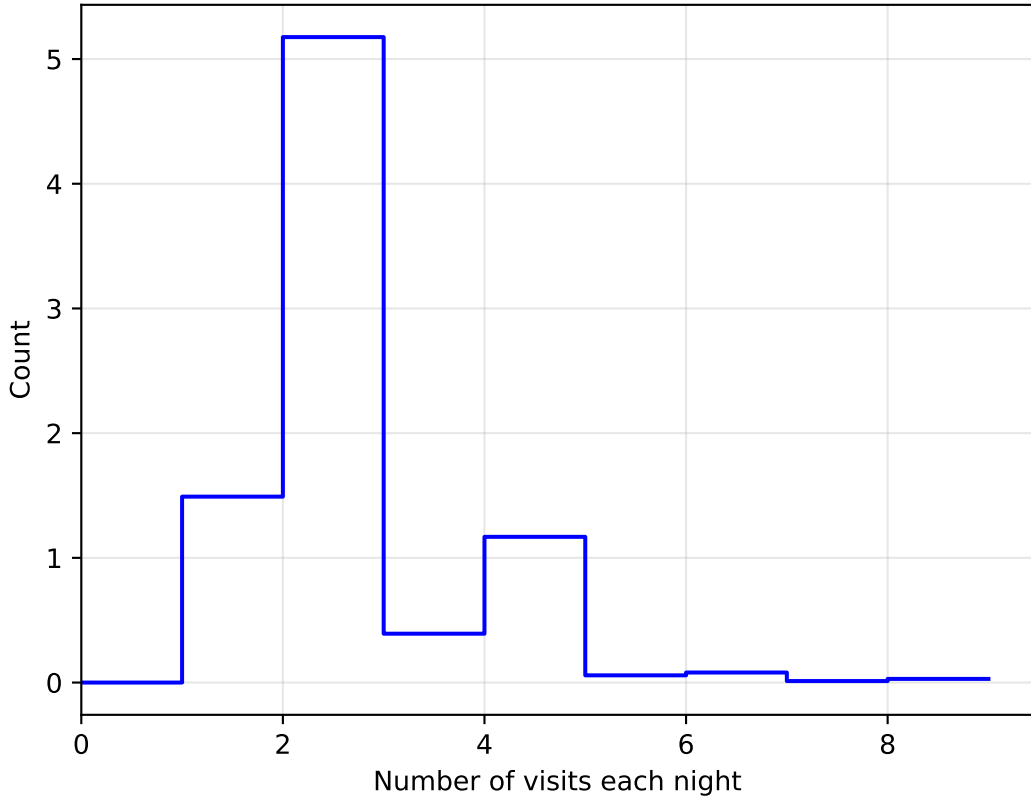
ddf_loaded_half_fl8_v3.4_10yrs WFD: NVisitsPerNight
