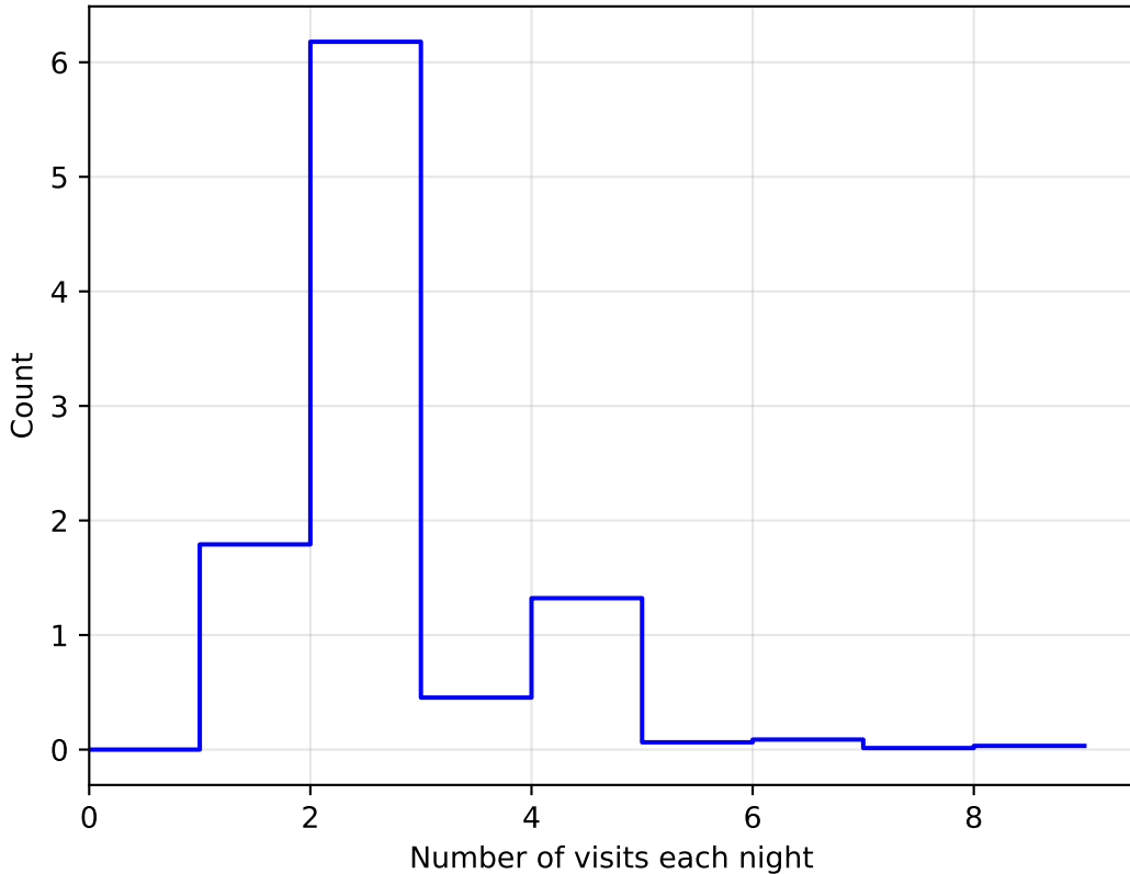
ddf_loaded_half_fl8_v3.4_10yrs All sky: NVisitsPerNight
