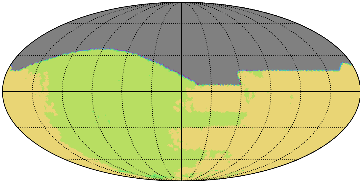
ddf_loaded_half_fl8_v3.4_10yrs All sky all bands: NSeasons
