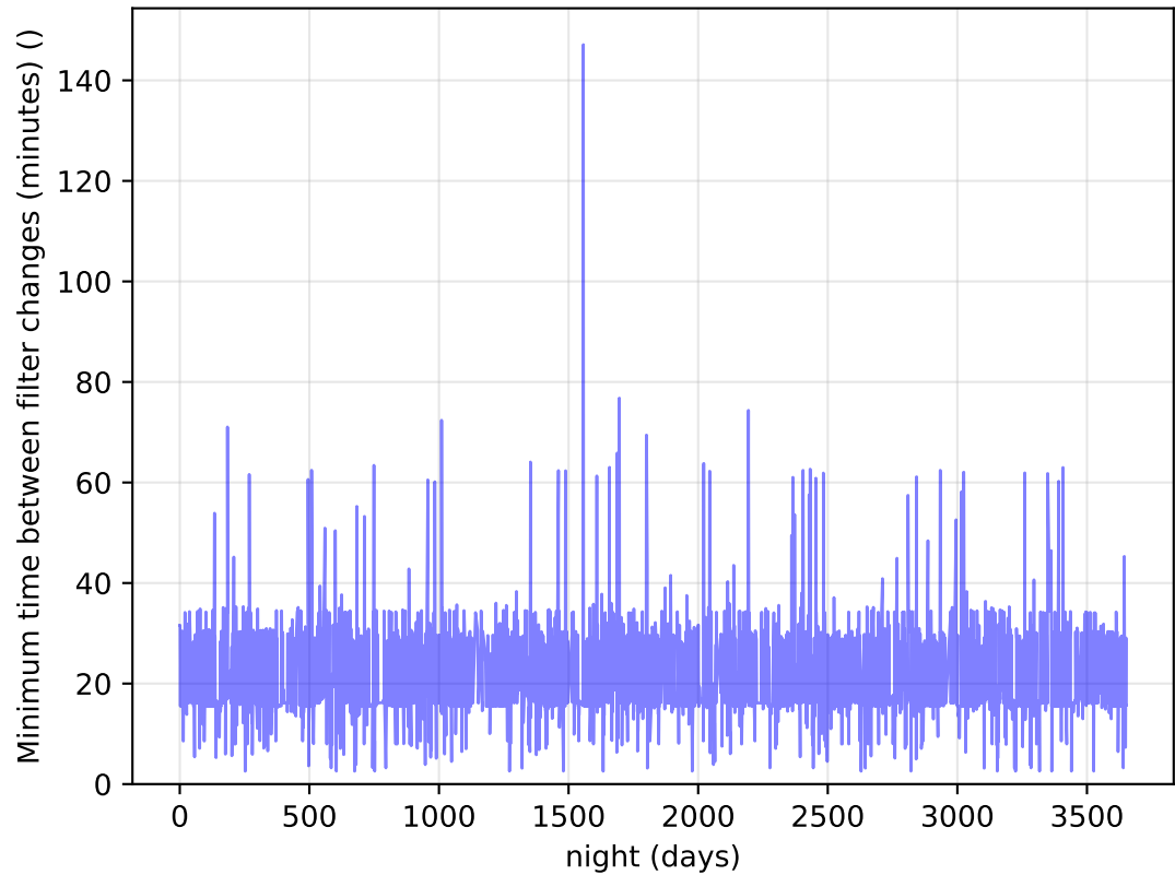
ddf_loaded_half_fl8_v3.4_10yrs Per Night: Minimum time between filter changes (minutes)
