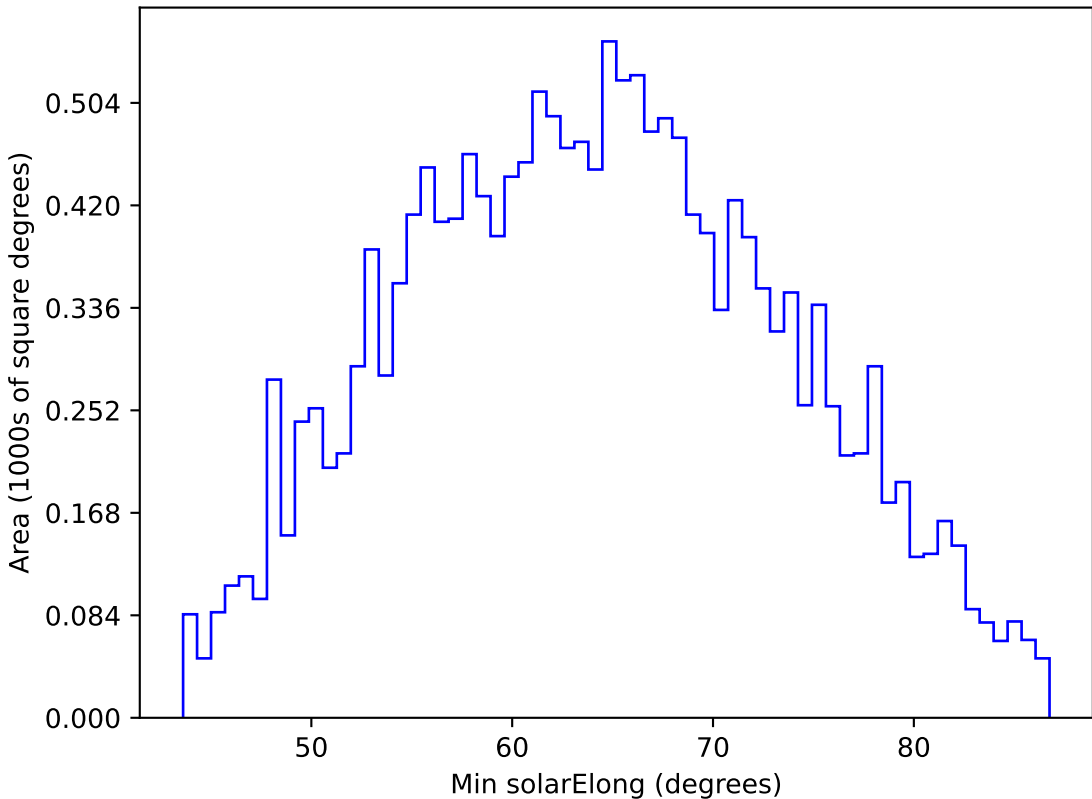
ddf_loaded_half_fl8_v3.4_10yrs WFD y band: Min solarElong
