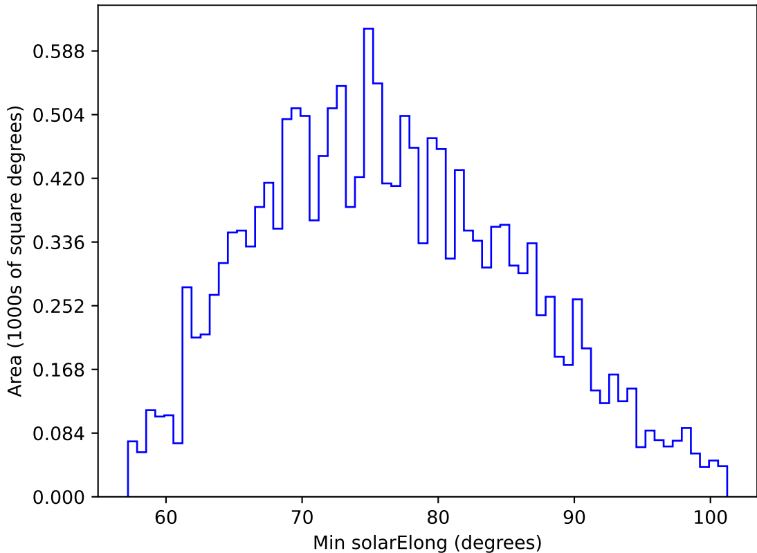
ddf_loaded_half_fl8_v3.4_10yrs WFD u band: Min solarElong
