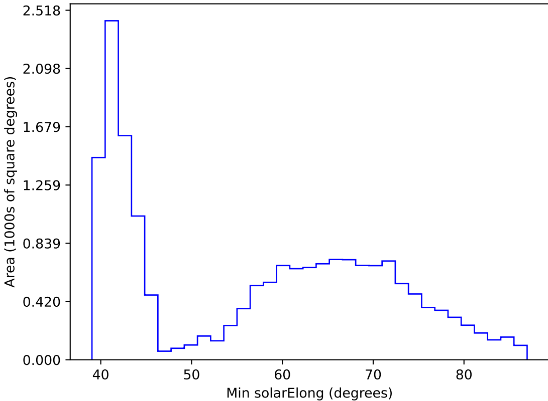
ddf_loaded_half_fl8_v3.4_10yrs WFD r band: Min solarElong
