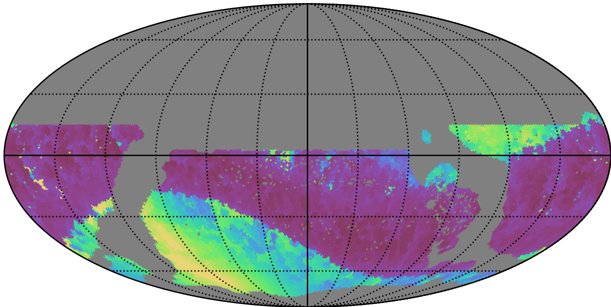
ddf_loaded_half_fl8_v3.4_10yrs WFD i band: Min solarElong
