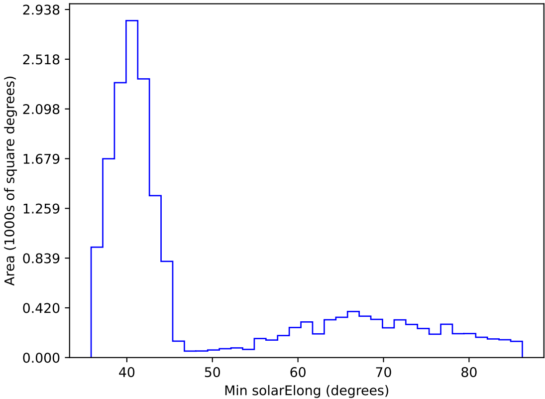
ddf_loaded_half_fl8_v3.4_10yrs WFD i band: Min solarElong
