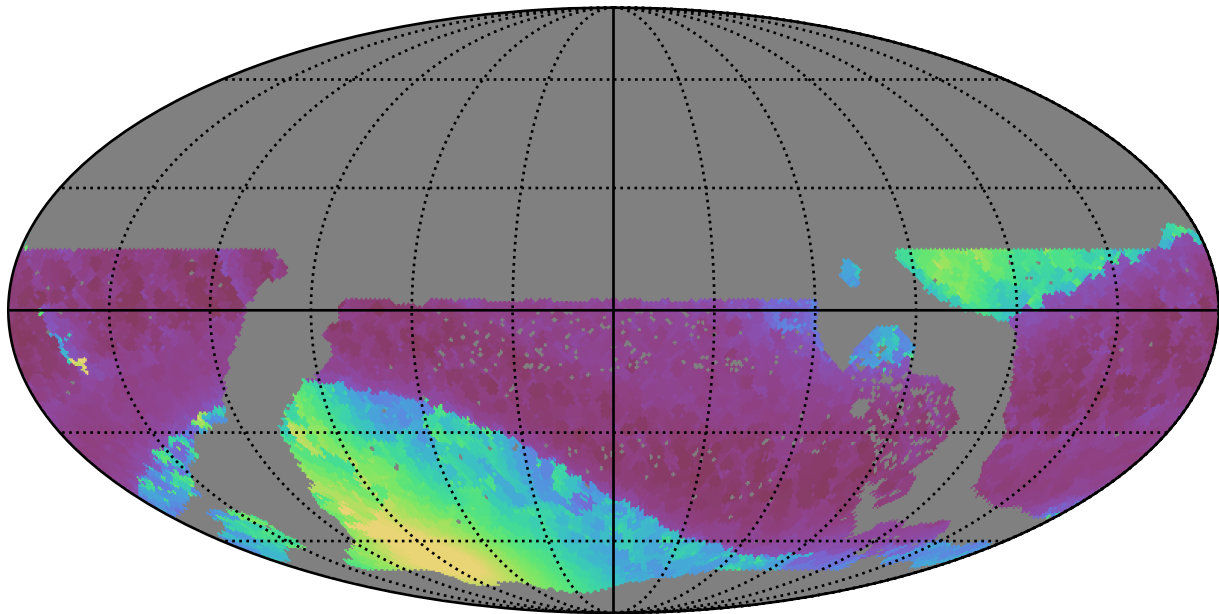
ddf_loaded_half_fl8_v3.4_10yrs WFD all bands: Min solarElong
