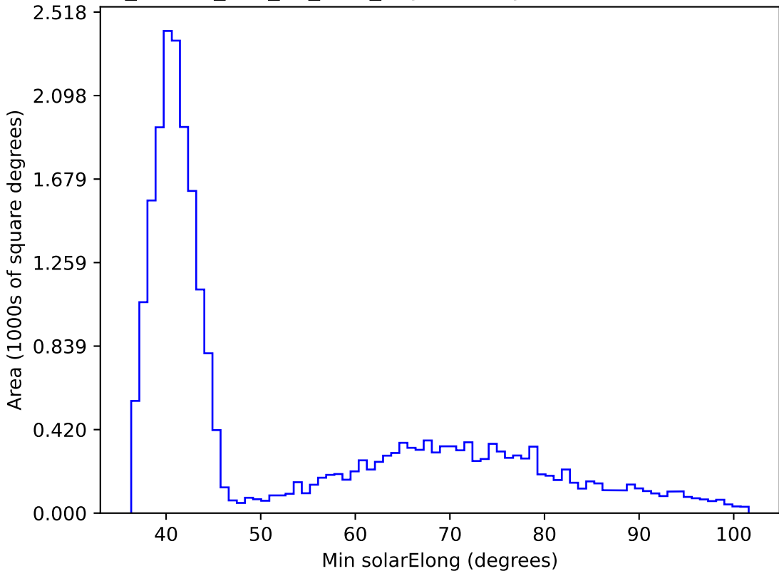
ddf_loaded_half_fl8_v3.4_10yrs All sky z band: Min solarElong
