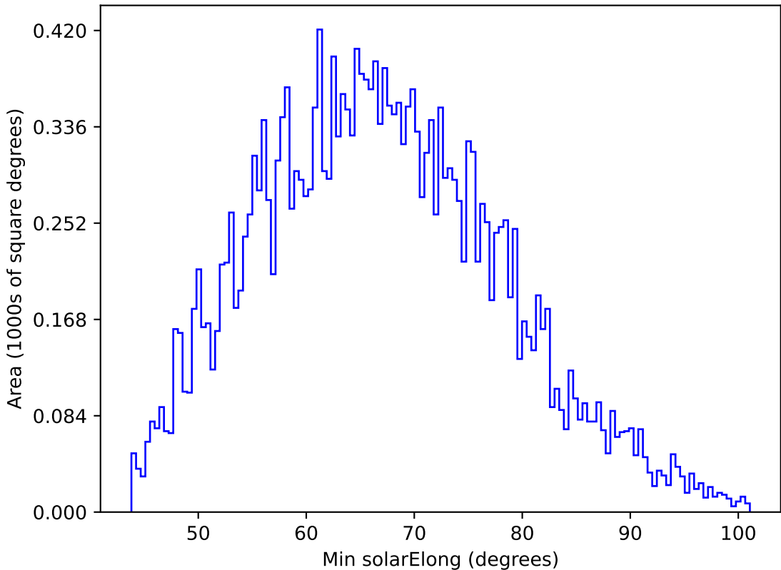
ddf_loaded_half_fl8_v3.4_10yrs All sky y band: Min solarElong
