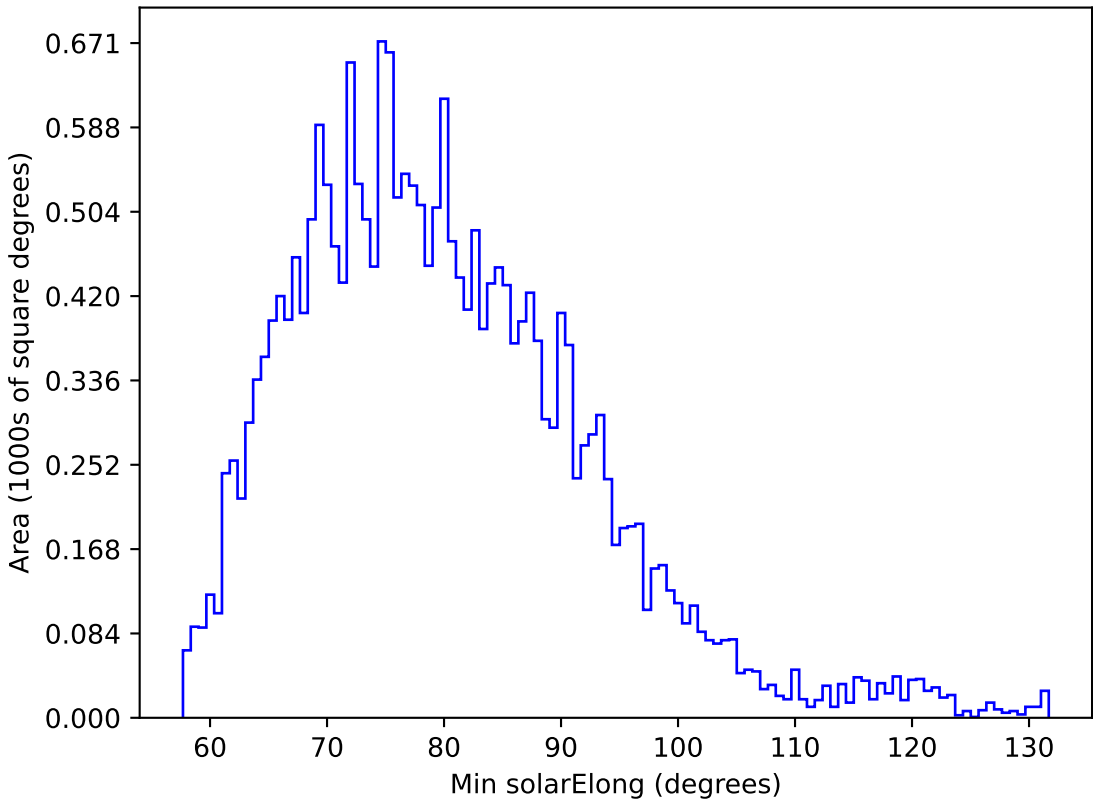
ddf_loaded_half_fl8_v3.4_10yrs All sky u band: Min solarElong
