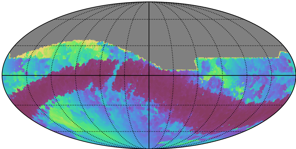
ddf_loaded_half_f18_v3.4_10yrs All sky r band: Min solarElong
