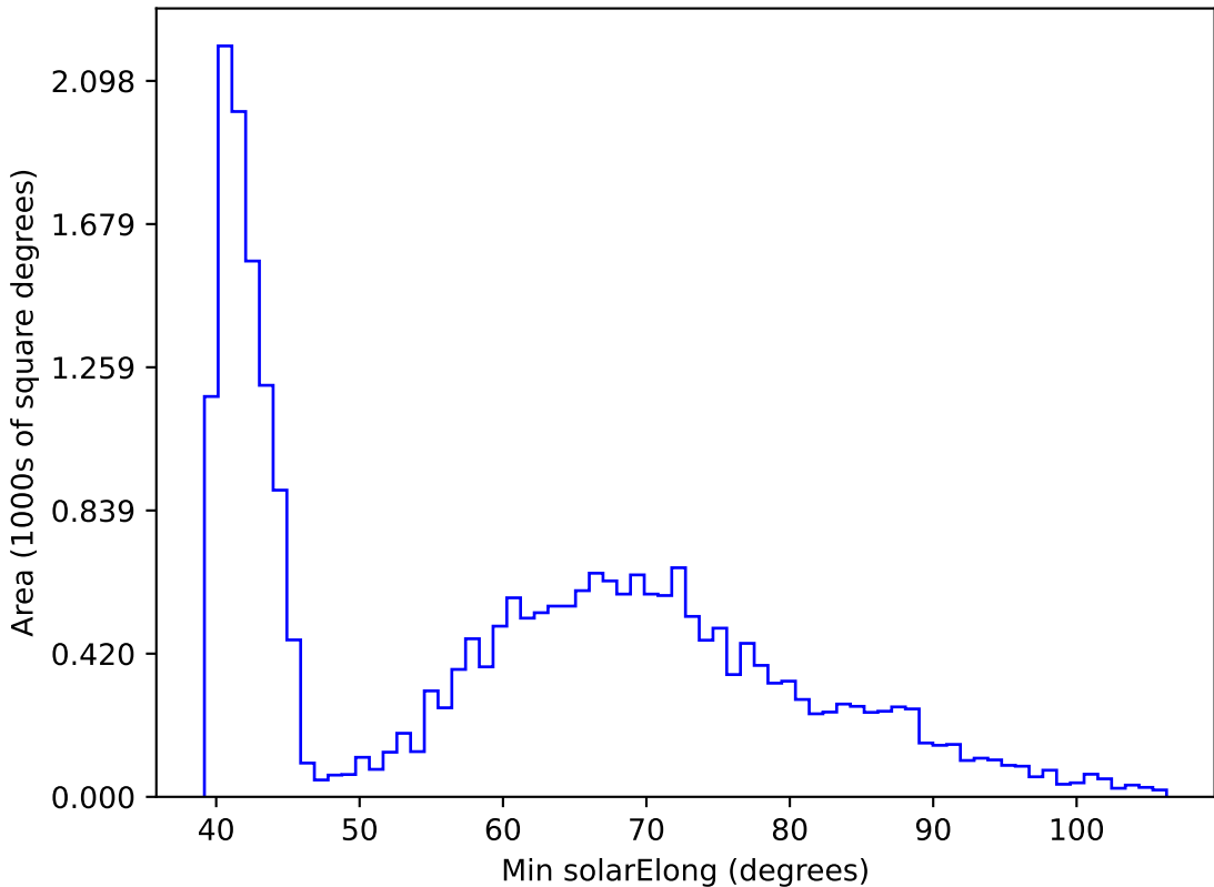
ddf_loaded_half_fl8_v3.4_10yrs All sky r band: Min solarElong
