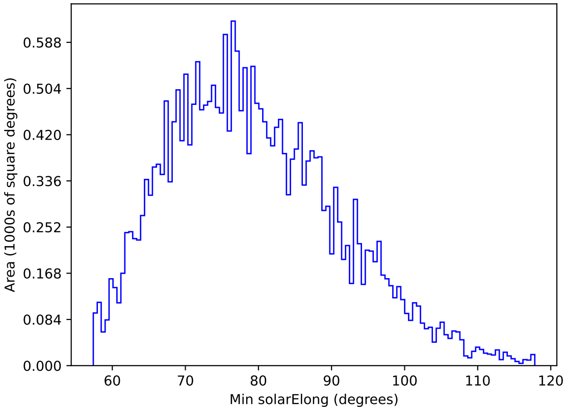
ddf_loaded_half_fl8_v3.4_10yrs All sky g band: Min solarElong
