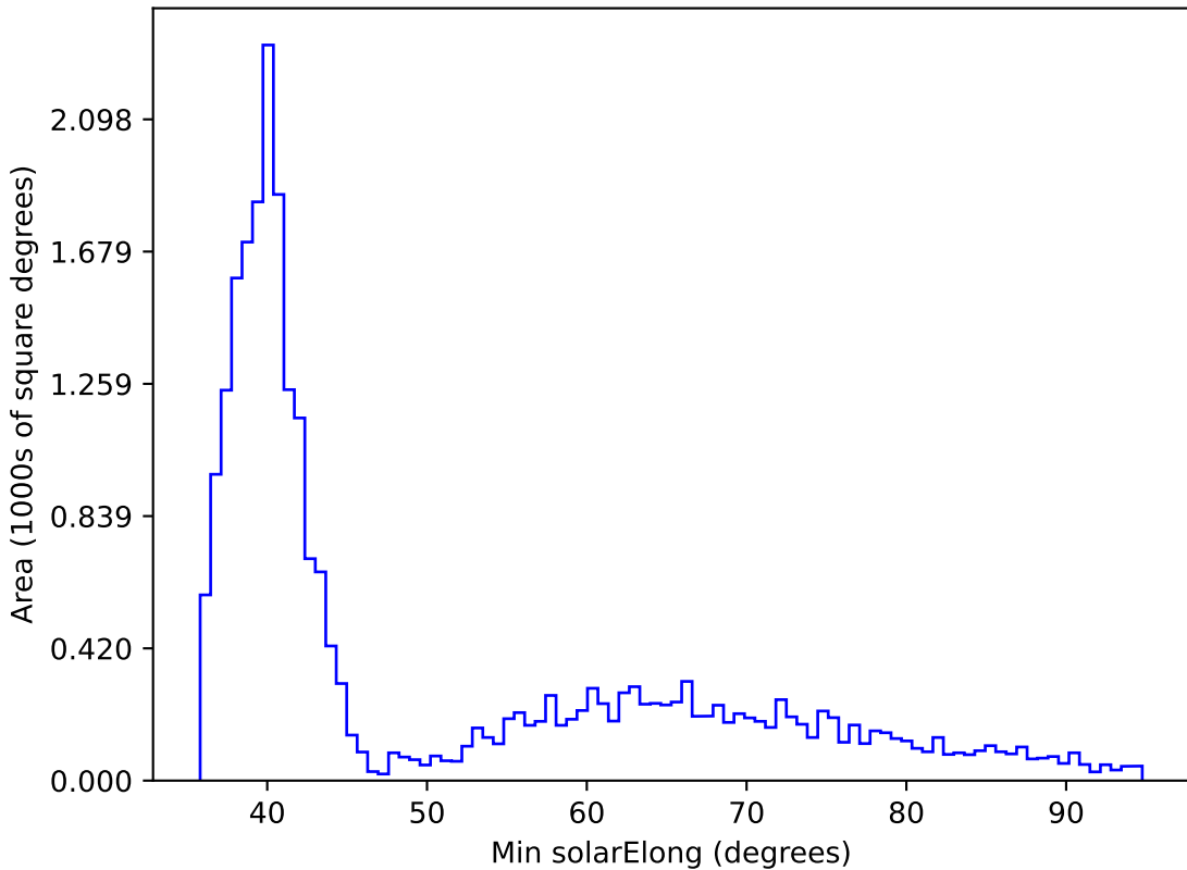
ddf_loaded_half_fl8_v3.4_10yrs All sky all bands: Min solarElong
