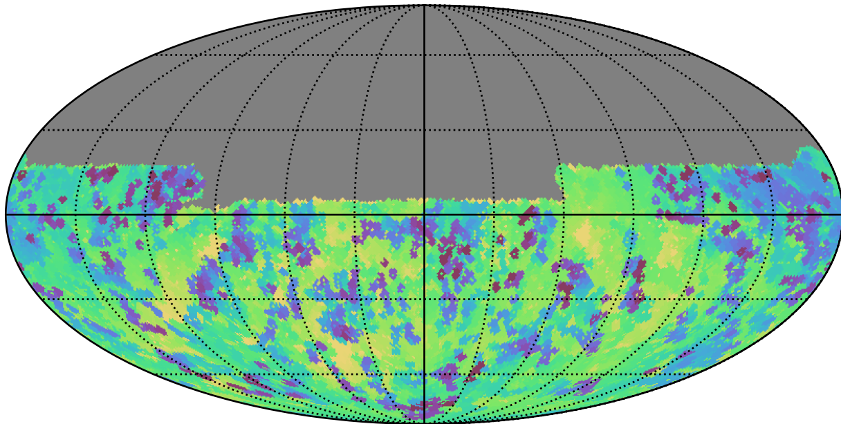
ddf_loaded_half_fl8_v3.4_10yrs Yr 1 y band: Min skyBrightness
