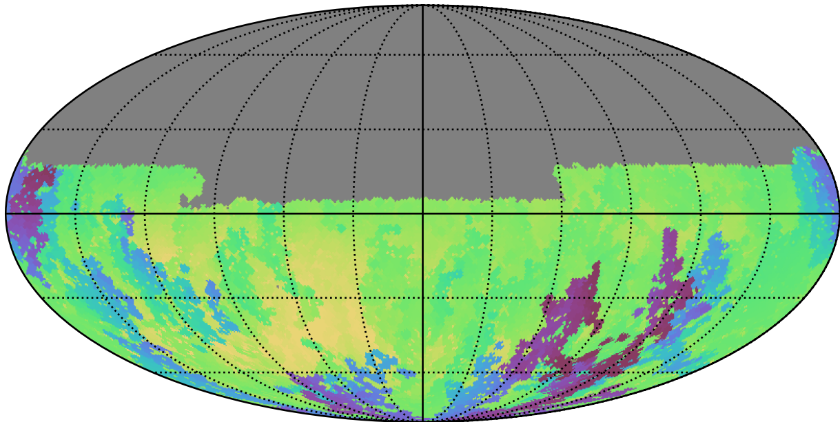
ddf_loaded_half_fl8_v3.4_10yrs Yr 1 u band: Min skyBrightness
