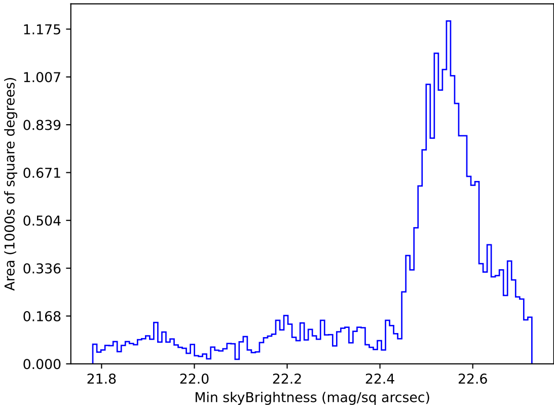
ddf_loaded_half_fl8_v3.4_10yrs Yr 1 u band: Min skyBrightness
