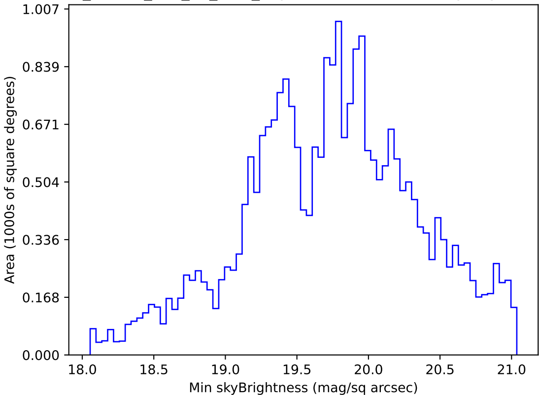
ddf_loaded_half_fl8_v3.4_10yrs Yr 1 r band: Min skyBrightness
