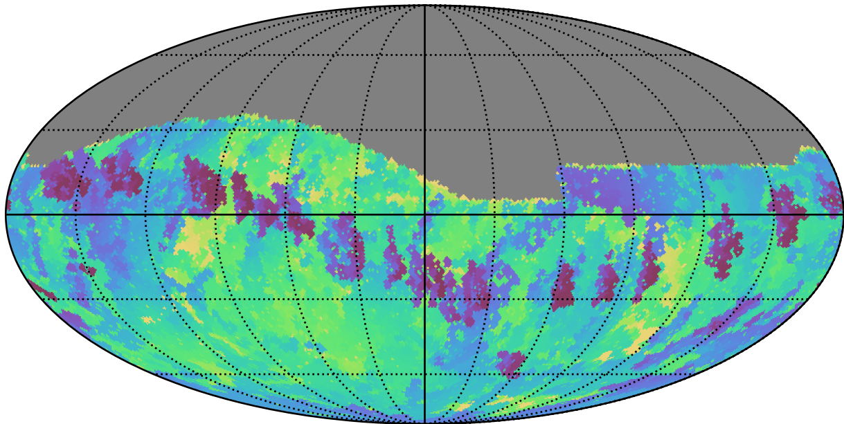
ddf_loaded_half_fl8_v3.4_10yrs Yr 1 i band: Min skyBrightness
