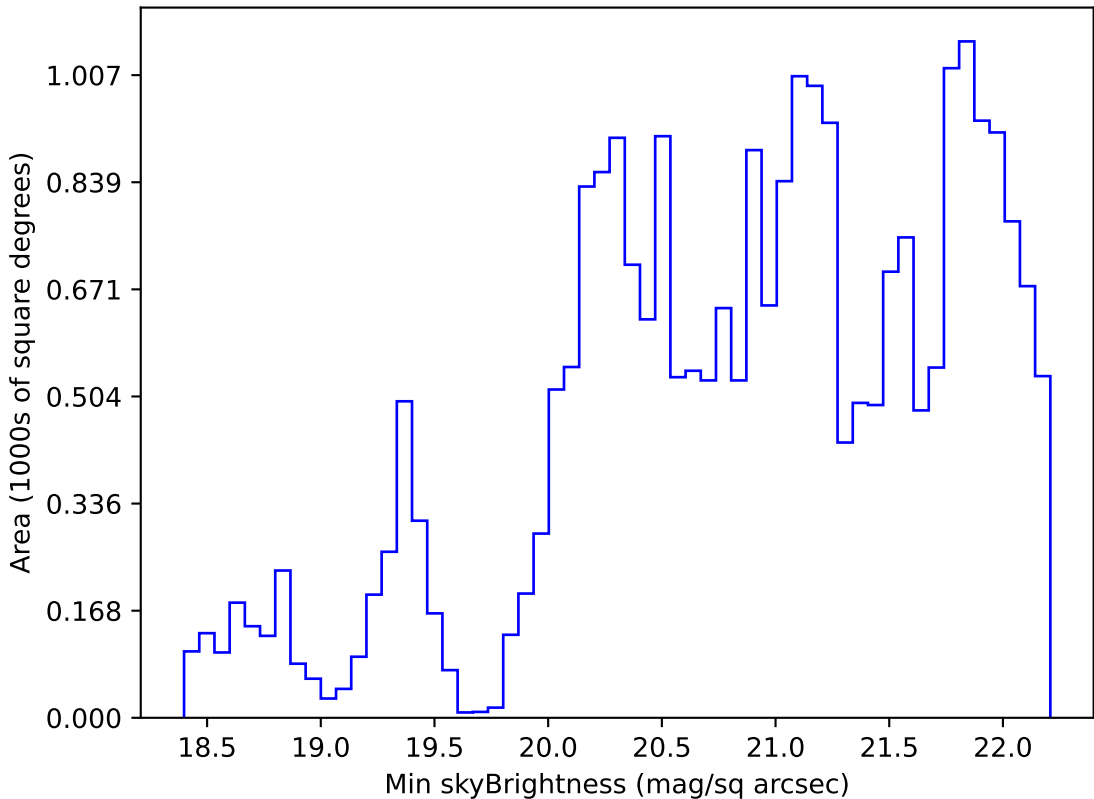
ddf_loaded_half_fl8_v3.4_10yrs Yr 1 g band: Min skyBrightness
