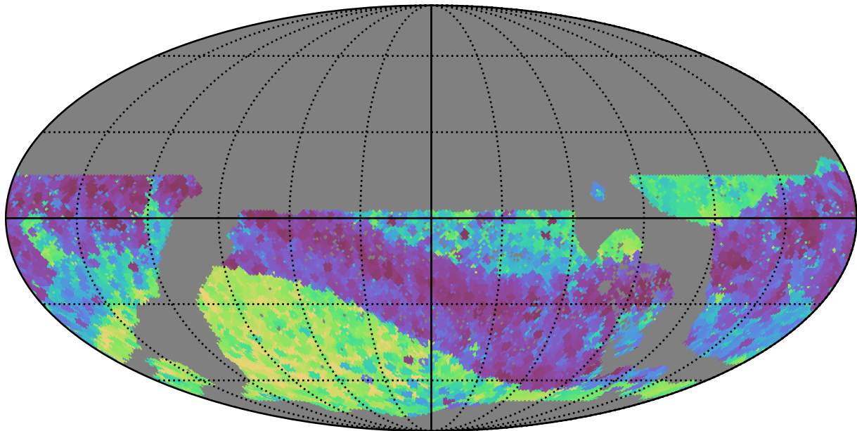
ddf_loaded_half_fl8_v3.4_10yrs WFD z band: Min skyBrightness
