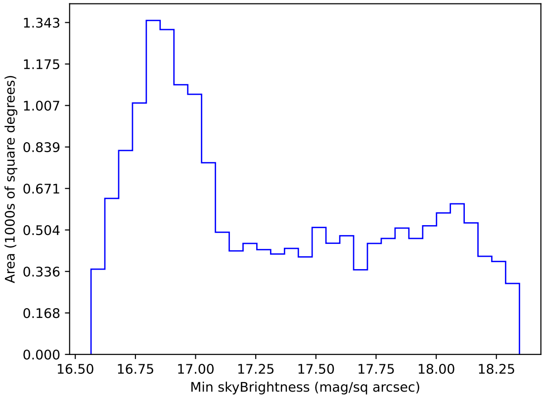
ddf_loaded_half_fl8_v3.4_10yrs WFD z band: Min skyBrightness
