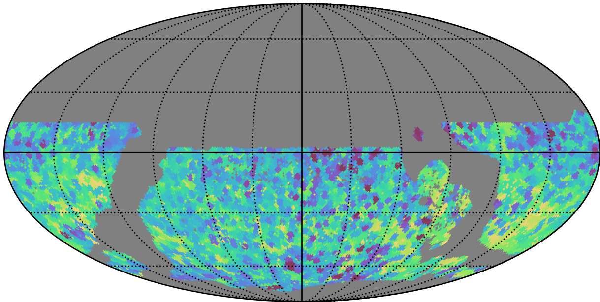
ddf_loaded_half_fl8_v3.4_10yrs WFD y band: Min skyBrightness
