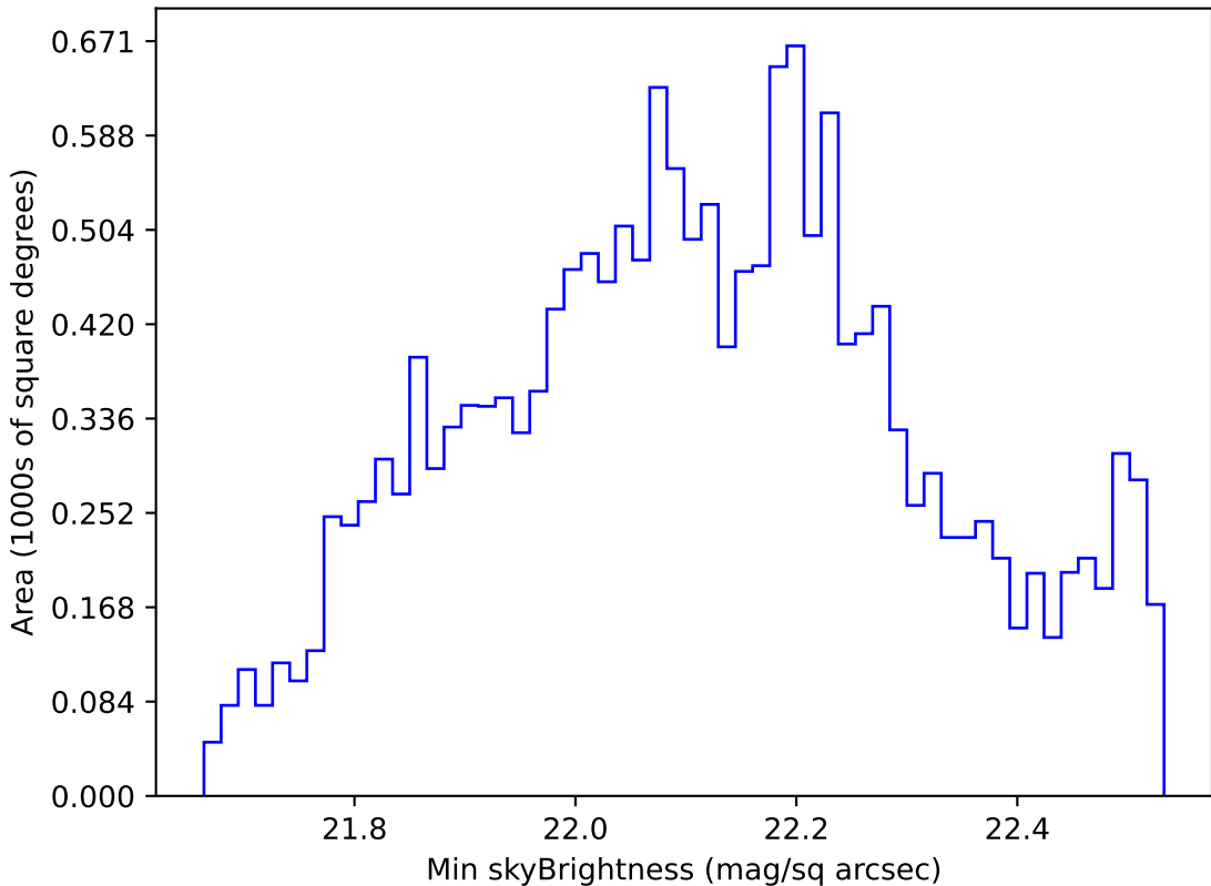
ddf_loaded_half_fl8_v3.4_10yrs WFD u band: Min skyBrightness
