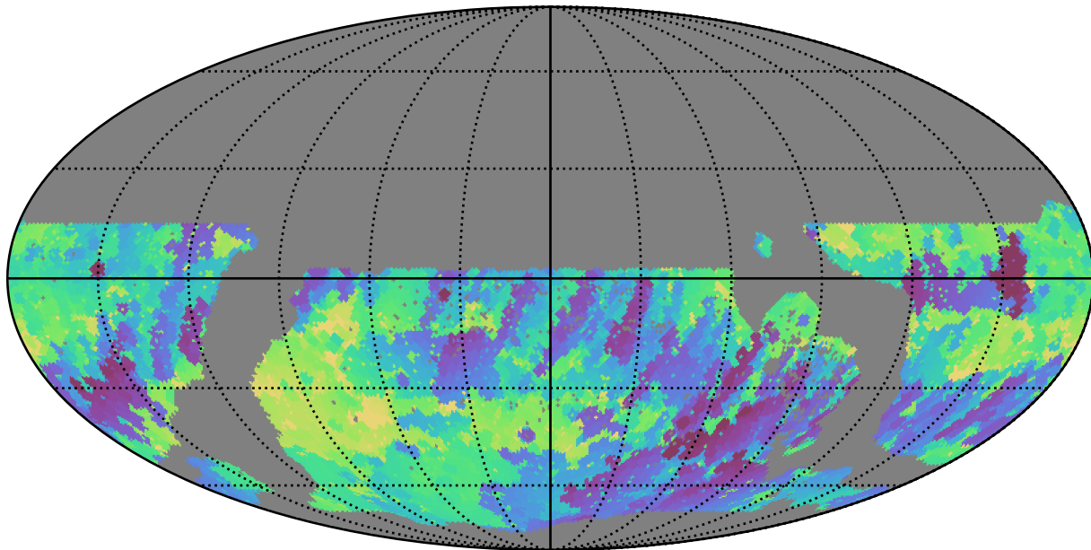
ddf_loaded_half_fl8_v3.4_10yrs WFD r band: Min skyBrightness
