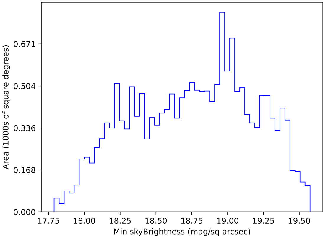
ddf_loaded_half_fl8_v3.4_10yrs WFD r band: Min skyBrightness
