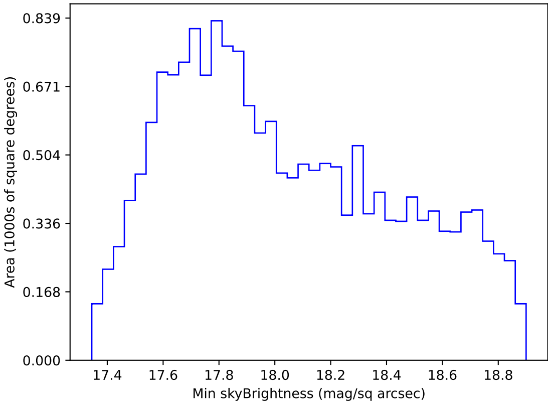
ddf_loaded_half_fl8_v3.4_10yrs WFD i band: Min skyBrightness
