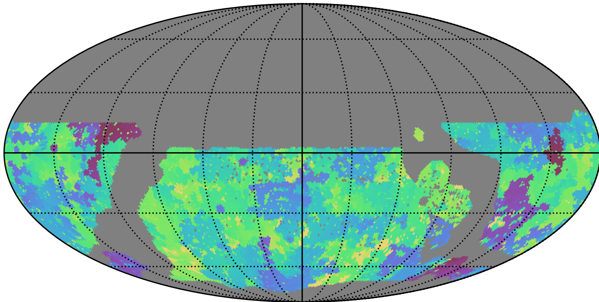
ddf_loaded_half_fl8_v3.4_10yrs WFD g band: Min skyBrightness
