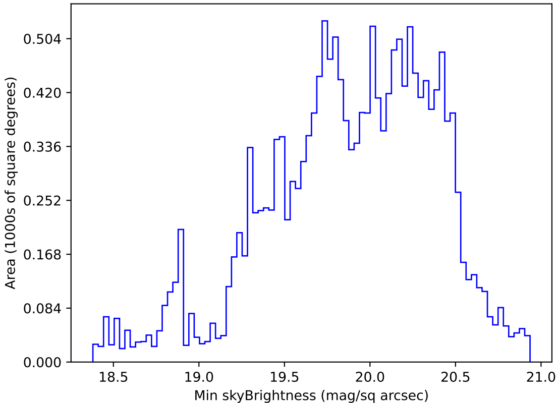
ddf_loaded_half_fl8_v3.4_10yrs WFD g band: Min skyBrightness
