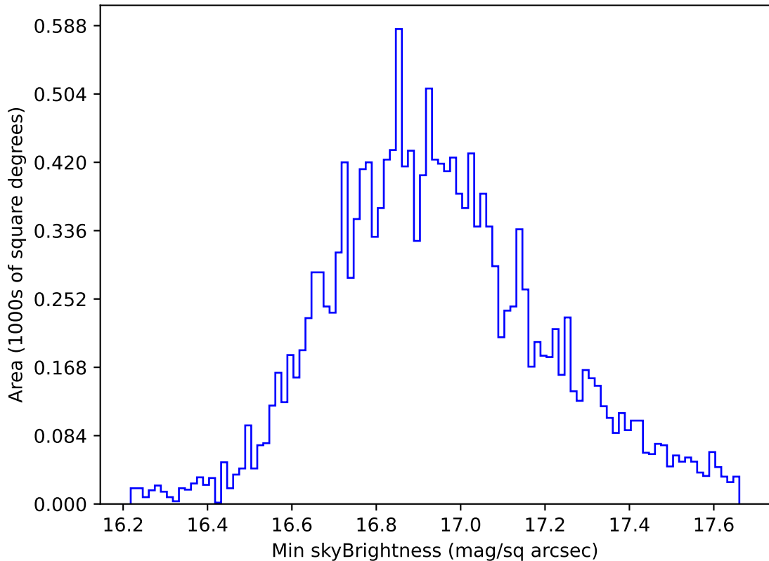
ddf_loaded_half_fl8_v3.4_10yrs WFD all bands: Min skyBrightness
