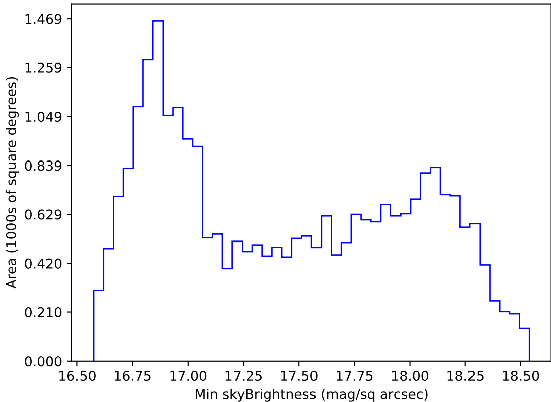
ddf_loaded_half_fl8_v3.4_10yrs All sky z band: Min skyBrightness
