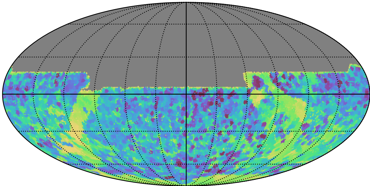
ddf_loaded_half_fl8_v3.4_10yrs All sky y band: Min skyBrightness
