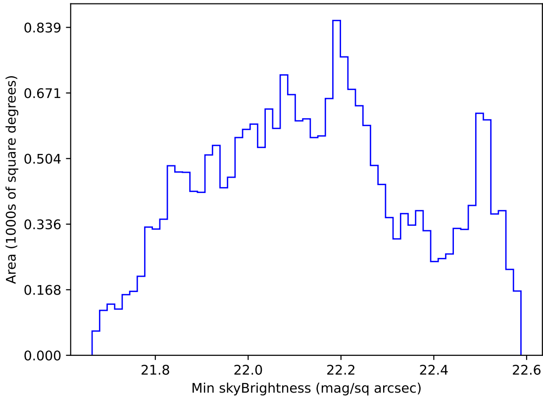
ddf_loaded_half_fl8_v3.4_10yrs All sky u band: Min skyBrightness
