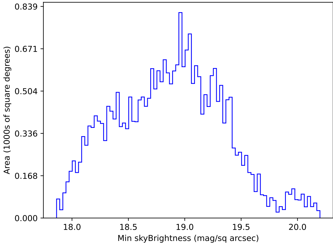
ddf_loaded_half_fl8_v3.4_10yrs All sky r band: Min skyBrightness
