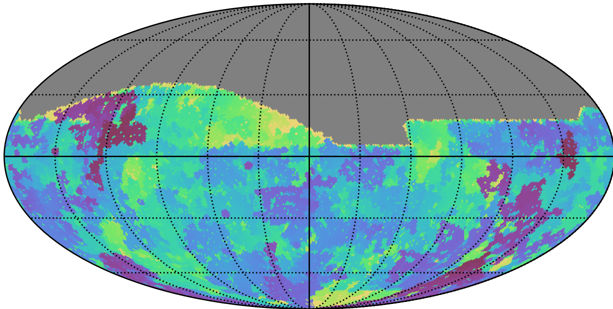
ddf_loaded_half_fl8_v3.4_10yrs All sky g band: Min skyBrightness
