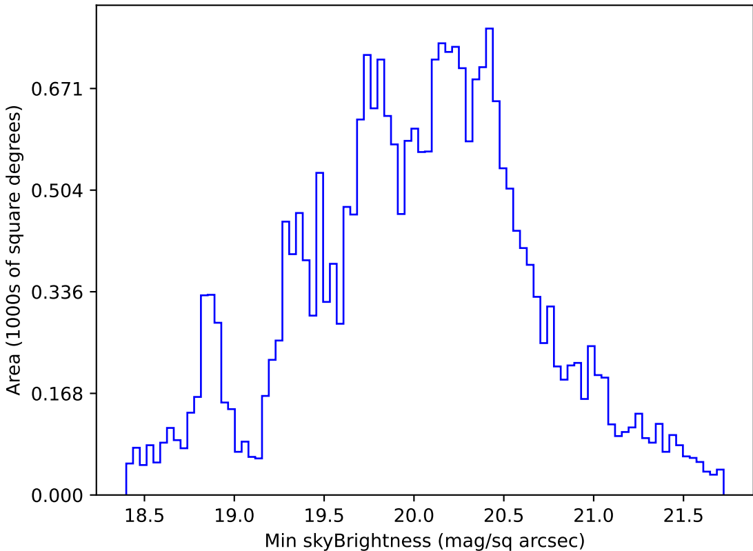
ddf_loaded_half_fl8_v3.4_10yrs All sky g band: Min skyBrightness
