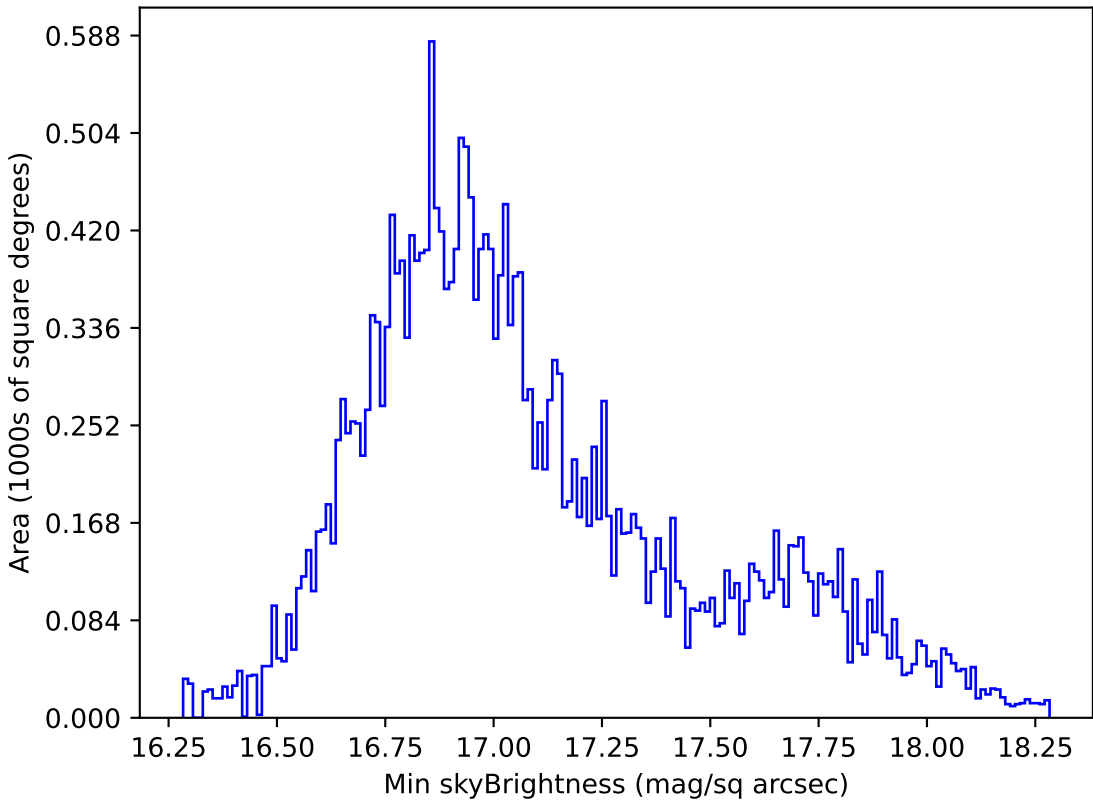
ddf_loaded_half_fl8_v3.4_10yrs All sky all bands: Min skyBrightness
