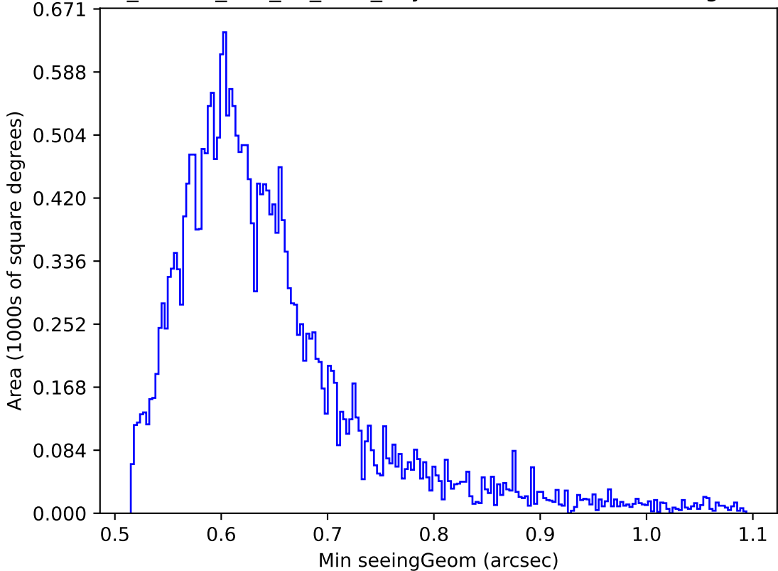
ddf_loaded_half_f18_v3.4_10yrs Yr 1 z band: Min seeingGeom
