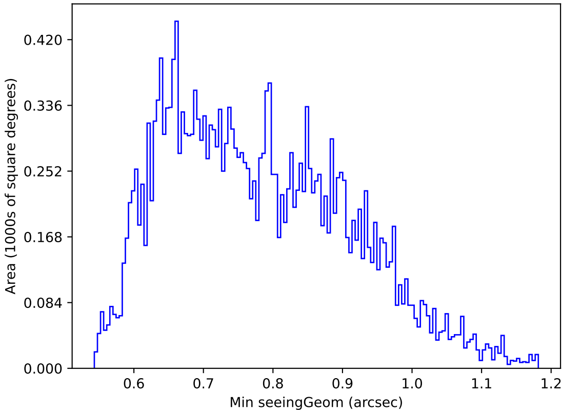
ddf_loaded_half_fl8_v3.4_10yrs Yr 1 u band: Min seeingGeom
